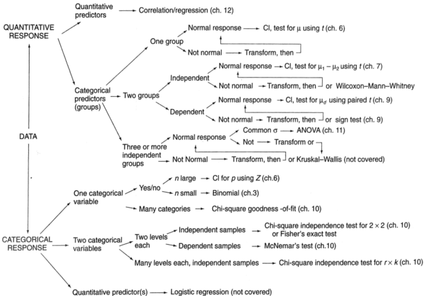
Figure 13.1 A flowchart of inference methods
