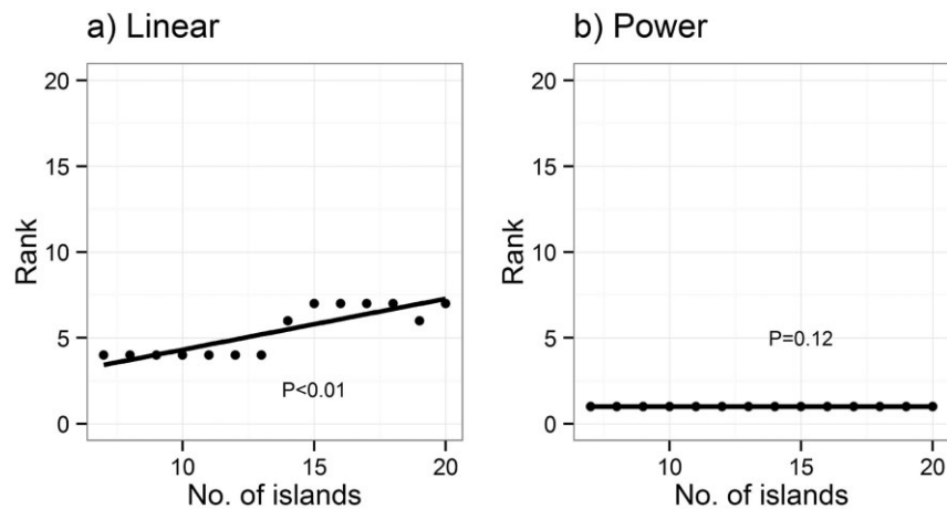
Figure 2 Change in model performance with the number of habitat islands in a dataset. Results for two models are displayed: (a) linear and (b) power models. The rank of a model refers to the model selection analysis in which 20 island species–area relationship models were compared using the AIC_c . A model rank was determined by standardizing the generality and efficiency criterion values (see ‘Materials and methods’), and adding these standardized values together. Thus, rank 1 refers to the model with the largest (larger values indicating a better performance) sum of standardized generality and efficiency values. Model ranks were first determined for all datasets with four or more islands, and then for all datasets with five or more islands, and so on, iteratively up to datasets with 20 or more islands. The linear model rank results were chosen as this was the model with the biggest change in model rank with the number of islands in a dataset. A linear regression line was fitted through the points and we tested to see if the slope of the line was significantly different from zero.
