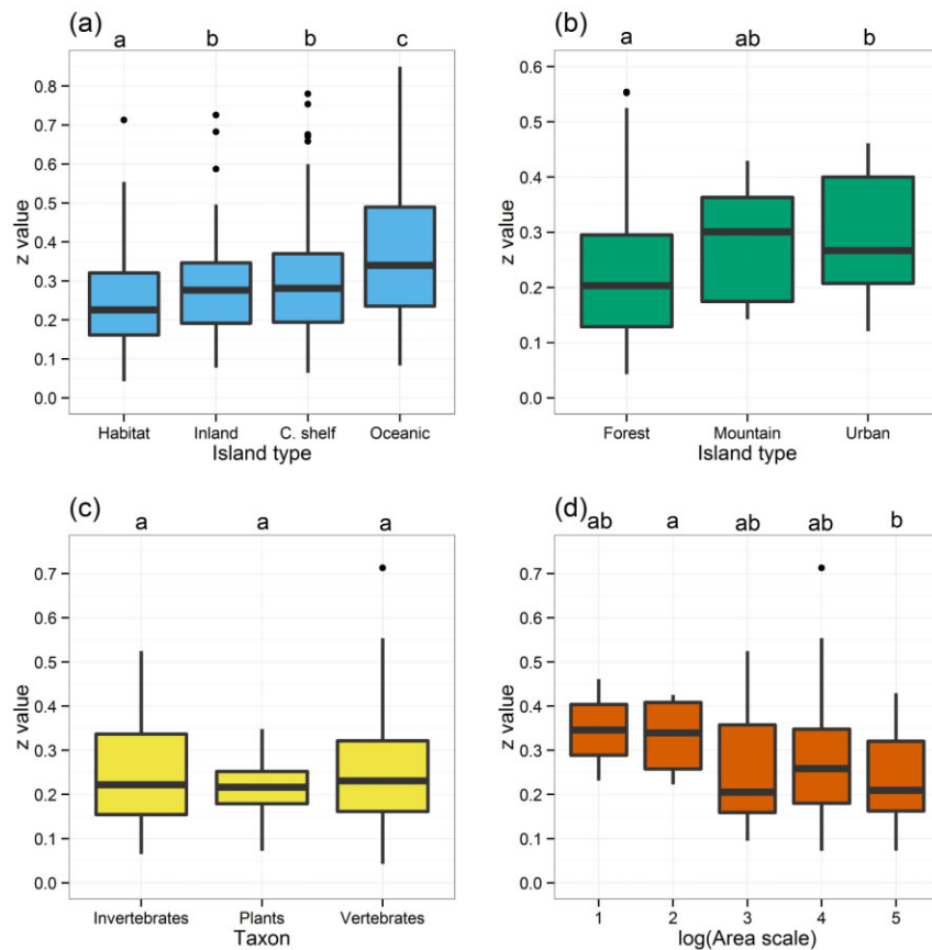
Figure 3 Variation in the z parameter of the power (log–log) model across (a) all island types, (b) different habitat island types, (c) different major taxa, and (d) area scale (log transformed). Note that (b)–(d) were calculated using only habitat island datasets. For all plots, only datasets with significant z -values ( P < 0.05 ) were included. For reasons of clarity, the boxplots were constructed after omitting the small number of z -values < 0 (all subsequent statistics were performed using the full set of data). Thus, in (a) there were 132 habitat island, 125 oceanic island, 58 inland water-body ('Inland') and 277 continental-shelf island datasets ('C. shelf'). In (b) there were 75 forest, 12 mountaintop and 21 urban habitat island datasets. In (c) there were 26 invertebrate, 20 plant and 86 vertebrate datasets. Area scale was calculated as the area of the largest island in a dataset divided by the area of the smallest island. Area scales larger than five have been omitted. The boxplots display the median (thick black line) and the first and third quartiles (thin black box). The whiskers extend from the hinge to the highest value that is within 1.5 multiplied by the interquartile range of the hinge. Outliers are indicated by solid dots. Significant differences in z -values between dataset categories are displayed as different lowercase letters above the boxplots. Values that do not significantly differ between categories have the same lowercase letters.
