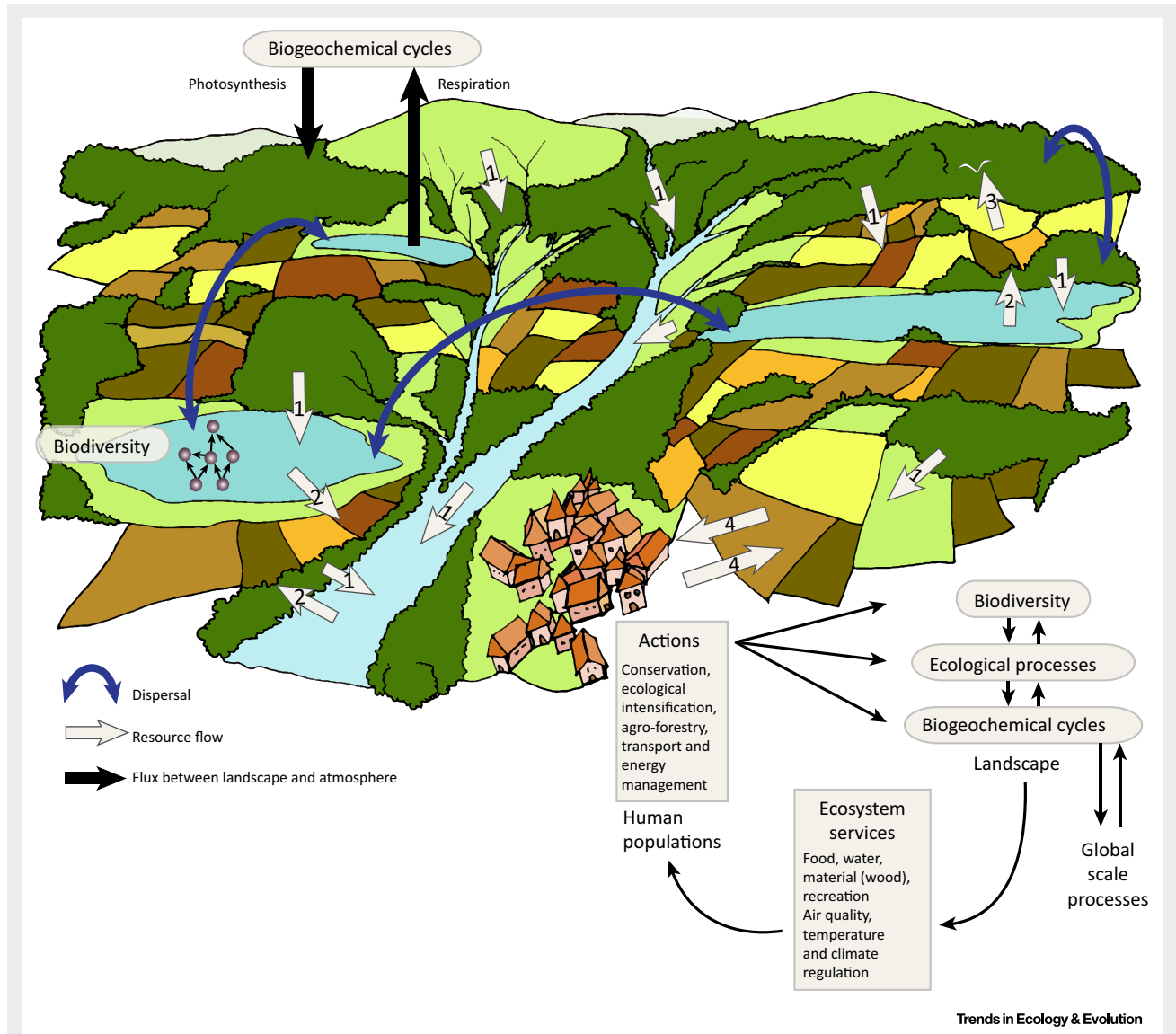
Figure 1. Spatial Dynamics at the Landscape Scale. Both flows of dispersal (curve blue arrows) and resource (white arrows) coupled different types of habitat patches in the landscape, thereby inducing contrasting meta-ecosystem dynamics at regional and local scales, respectively. Flows of resources can be driven by physical forces such as gravity, wind, or water current (arrows 1), by animal movement such as insect emergence (arrows 2) or consumer foraging (arrow 3 next to a white bird), or by human transport (arrows 4). These flows affect biodiversity (e.g., denoted by a food web in a lake) and ecosystem processes (productivity and recycling), which themselves affect global cycles in different ways: example of the carbon cycle depicted by wide black arrows, with net carbon uptake by a forest patch and net carbon release to the atmosphere by a lake. Human populations benefit from ecosystem services provided by the landscape (right box), and human actions (left box) conducted at the landscape scale modulate biodiversity and ecosystem functioning, and ultimately biogeochemical cycles, which in turn induce the services.
