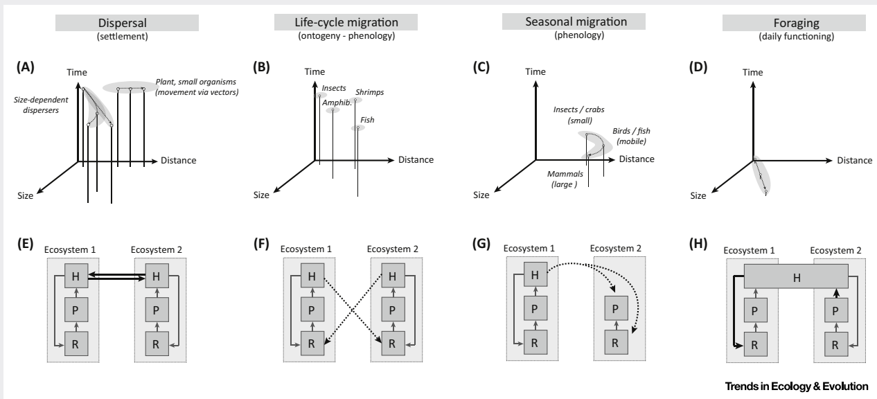
Figure 1. Scales of Organismal Movement Types and Effects on Meta-Ecosystem Dynamics. Top panels (A–D) show the qualitative relationships between organism size, the distance crossed for a given type of movement, and the time spent relative to the lifespan of the organism (inverse frequency). For instance, dispersal movement (A), or life-cycle migration (which corresponds to movement between contrasting habitats associated with specific ontogenic stages) (B), occur only once in a lifetime, whereas seasonal migration (C) occurs several times at regular intervals, and movement linked to foraging (D) occurs on a short time basis and multiple times during the life of an organism. The distance crossed during these movements might depend on the size and the mobility (e.g., flying ability) of the organisms, with larger or more mobile ones dispersing and migrating farther, or foraging on larger spatial scales (A–D) [70,71]. However, small organisms can also cross large distances through passive dispersal driven by air, or water currents, or larger organisms (A). Bottom diagrams (E–H) illustrate how spatial flows of an herbivore H (black arrows) driven by these different movement types might couple two ecosystems in which the herbivore feeds on a plant P, itself up-taking a resource R (grey boxes and arrows). In the meta-ecosystem framework, dispersal corresponds to movement among populations of the same species (E), whereas life-cycle movements represent added resources into the recipient ecosystem, since adults most often die immediately after reproducing (F). Dotted arrows denote that these flows are often as temporally specific pulses. In seasonal migrations, pulsed flows can be of a magnitude that constitutes a shift in the recipient community structure compared to otherwise prevailing local dynamics (G). Lastly, foraging activity can constitute a net flow from an ecosystem to another, even if the animal uses the whole landscape and does not perceive it as a structured meta-ecosystem (H).
