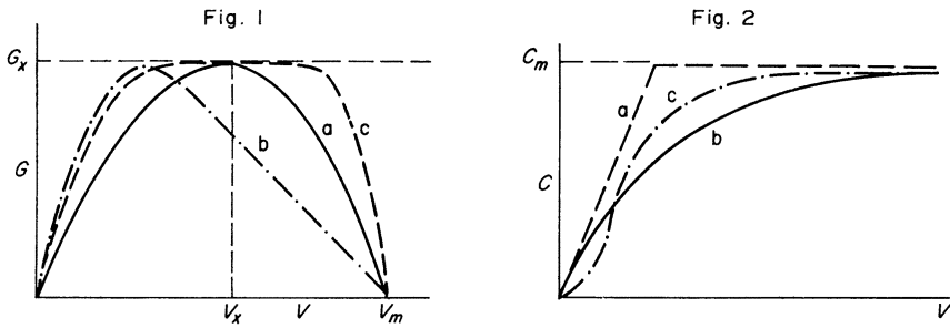
FIG. 1. Plant growth ( G ) as function of plant biomass ( V ). (a) Logistic growth; G_x —maximal growth, V_x —biomass at which growth is maximal. (b) and (c) Other possible curves.
