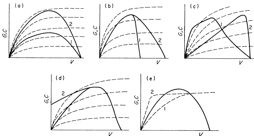
FIG. 11. The effects of plant characteristics on the combination of G(V) and C(V) . (a) Varying g and G_{max} . (b) Varying V_{max} . (c) Varying V_x , g , and the initial convexity of G(V) . (d) The effect of a residual plant biomass or growth potential. (e) Varying the level of V which allows herbivore consumption to be satiated.
