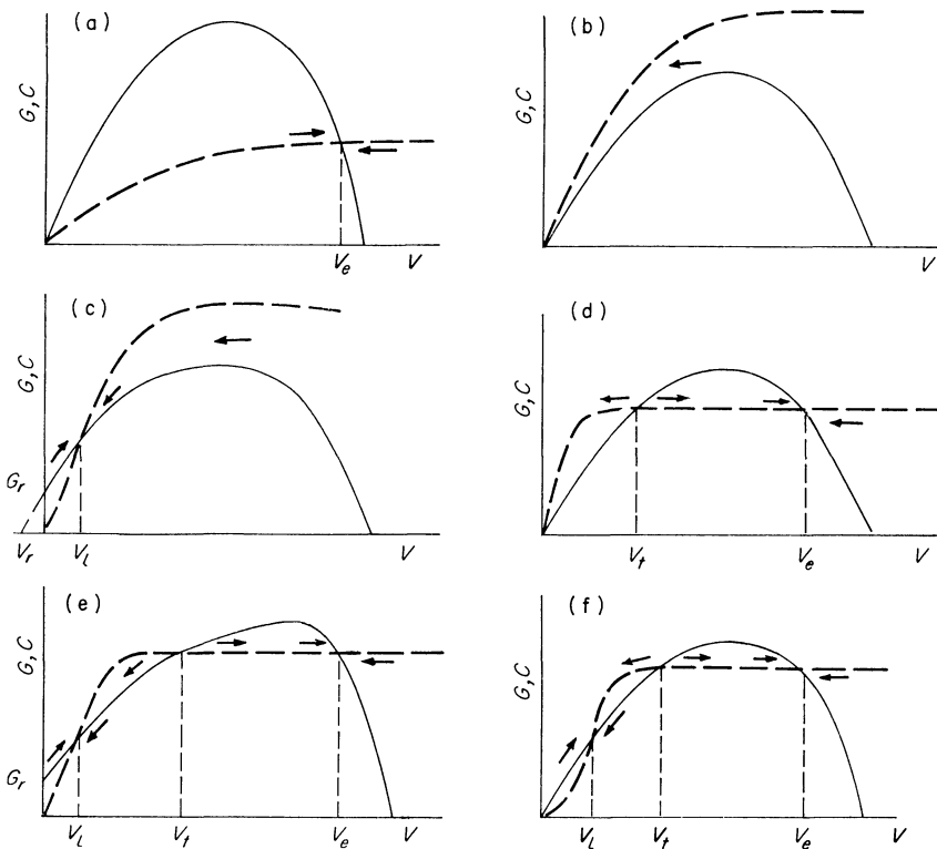
FIG. 5. Possible stability combinations of G - and C -curves at given H . (a) Undergrazed, stable steady-state ( V_e ). (b) Overgrazed to extinction. (c) Overgrazed to a low biomass steady-state ( V_i ); V_r —reserve (ungrazed) biomass, G_r —residual growth potential. (d) Steady-state and unstable turning point ( V_i ) to extinction. (e) Two steady-states ( V_e , V_i ) separated by turning point. (f) As (e), but caused by sigmoid C -curve, not by ungrazeable plant reserve.
