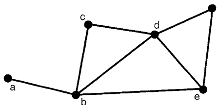
FIG. 1. An example of a graph defined by the sets of p = 6 nodes \{a, b, c, d, e, f\} and q = 8 edges \{ab, bc, be, bd, cd, de, df, ef\} .
