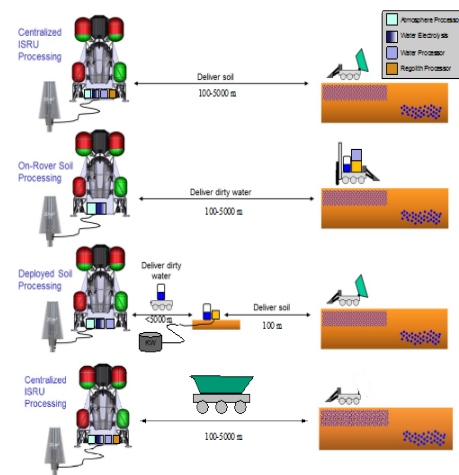
Figure 14: ISRU architecture concepts for resource acquisition and delivery.
