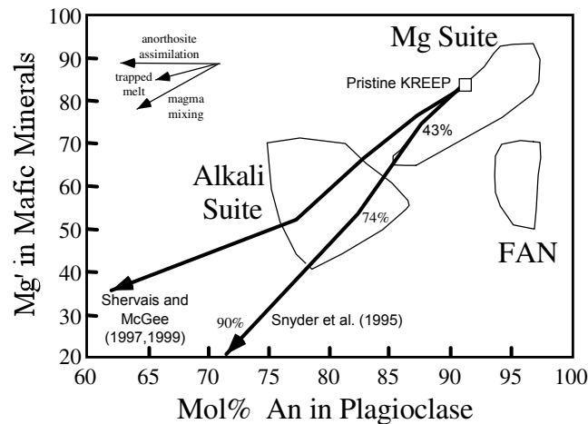
Figure 4.20. Anorthite content (An) in plagioclase vs. Mg' of coexisting mafic silicates for lunar highland plutonic rocks (modified after Warren 1986 and Snyder et al. 1995).
