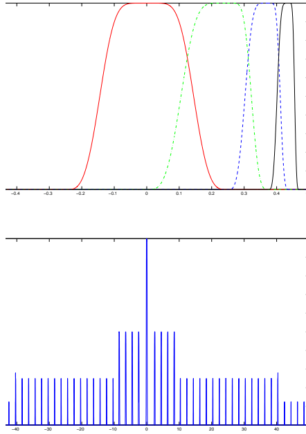
FIGURE 1. The functions h_i, 0 \leq i \leq 3 with \alpha = 1 on the top, and the function \widehat{\psi_{\alpha, \beta, n}} with \alpha = 1, \beta = 2 and n = 2 on the bottom.
