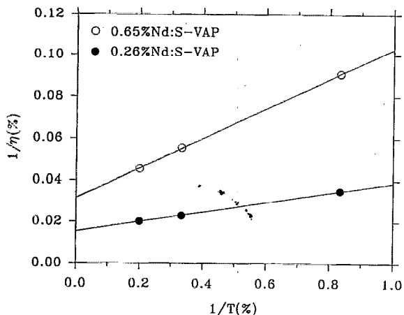
FIG. 11. Inverse slope efficiency versus inverse output coupling for 0.26% Nd 3+ and 0.65% Nd 3+ -doped S-VAP laser crystals when lasing at 1.065 μm.
